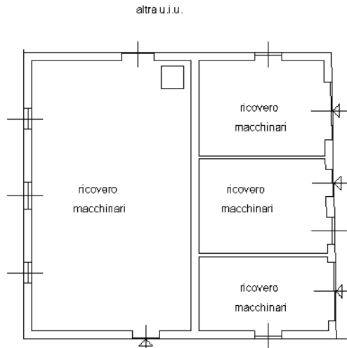
PIANO TERRA h285
